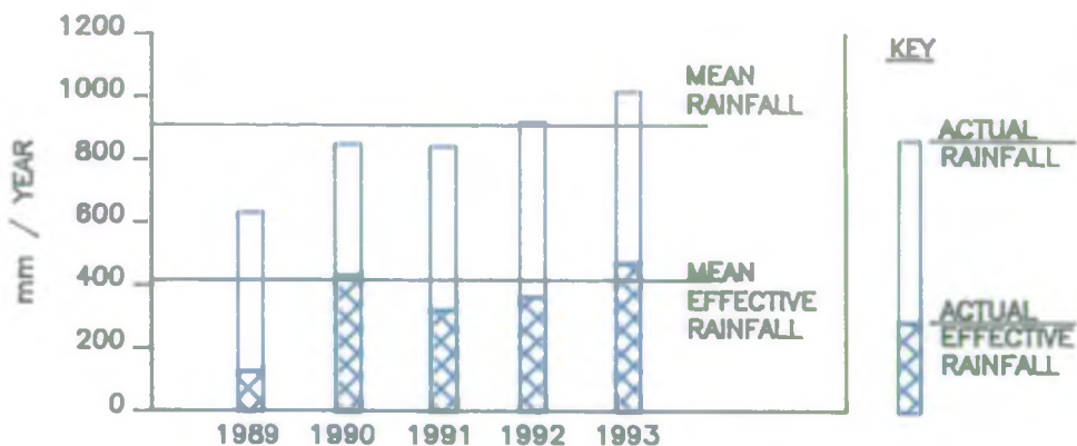
Annual Rainfall Record from Warnford Rainfall Station at SU627235 Actual Evapotranspiration Data from MORECS Database (Sq 182)
